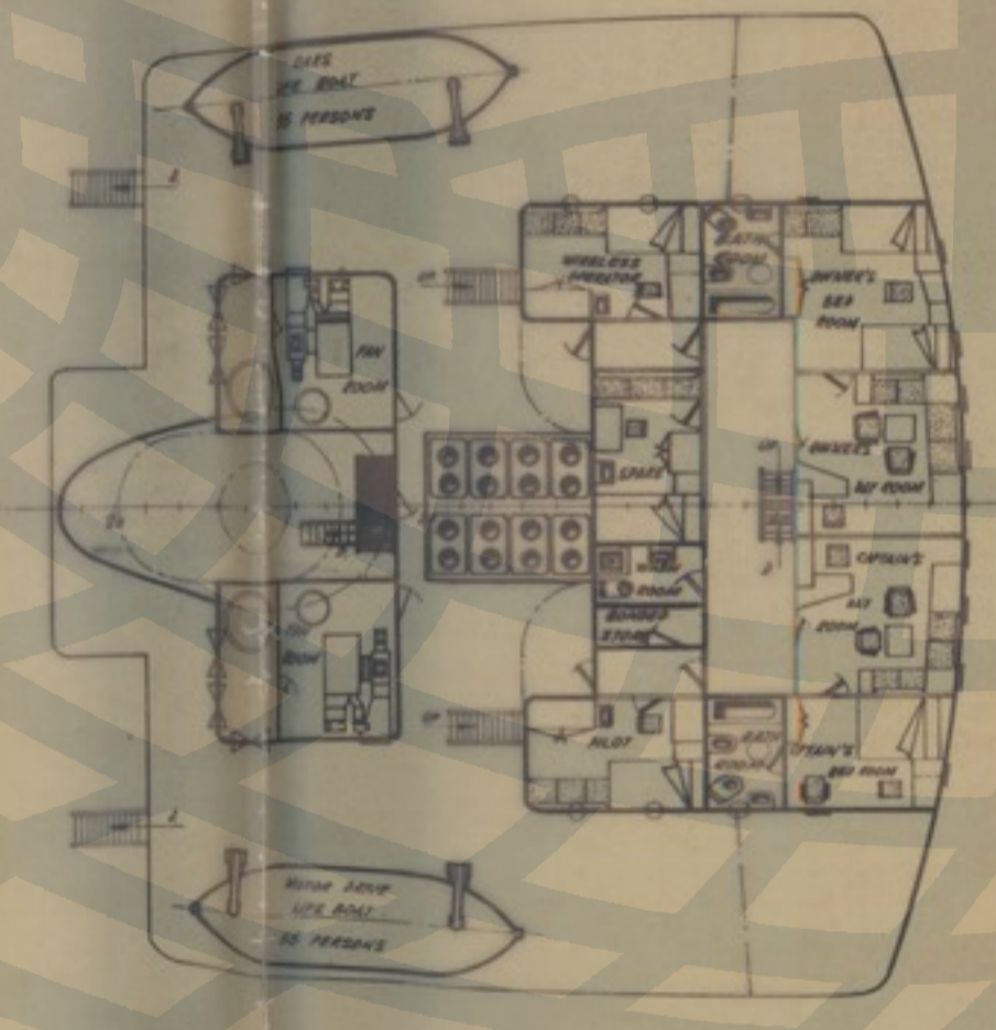
BOAT DECK
