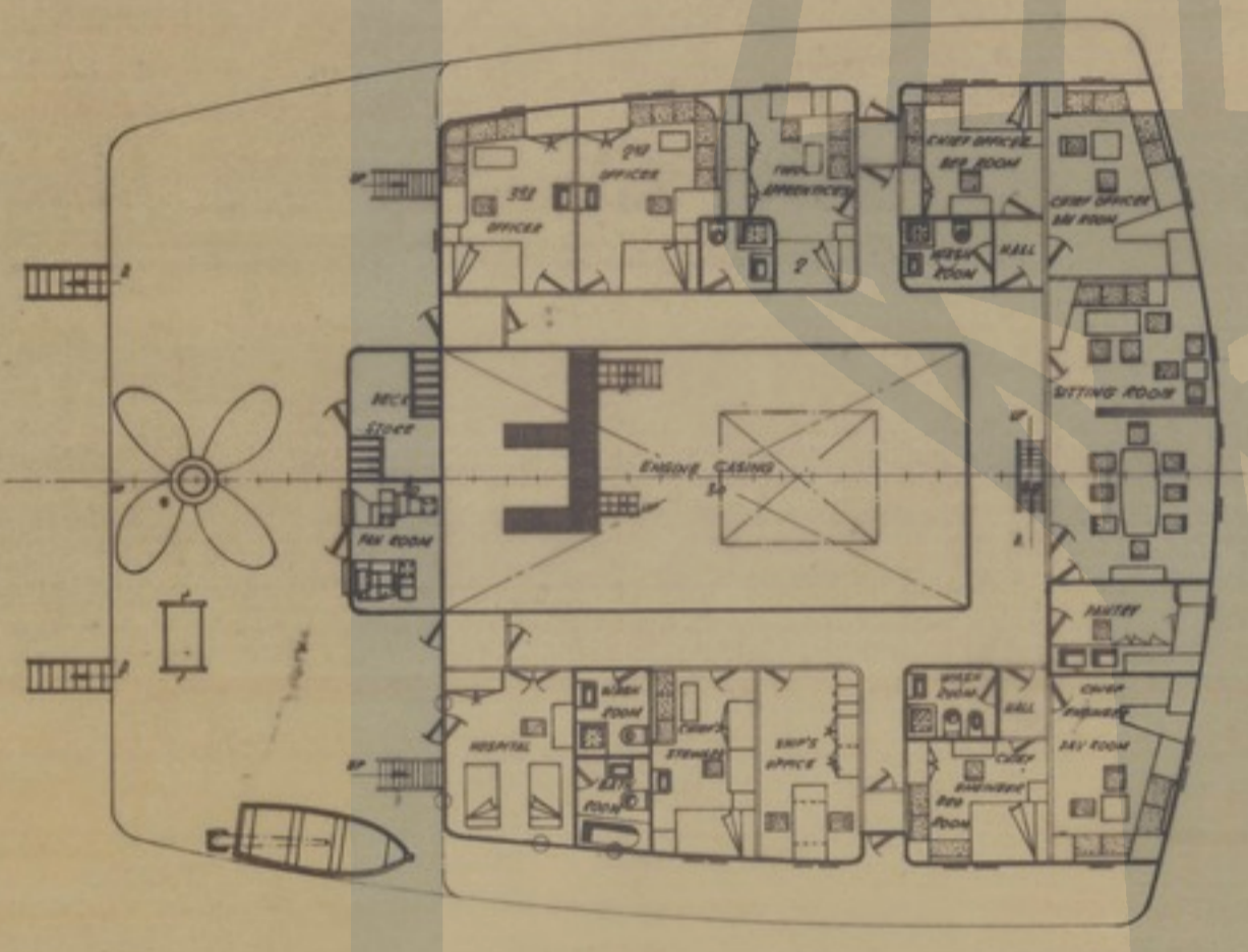
BRIDGE DECK
