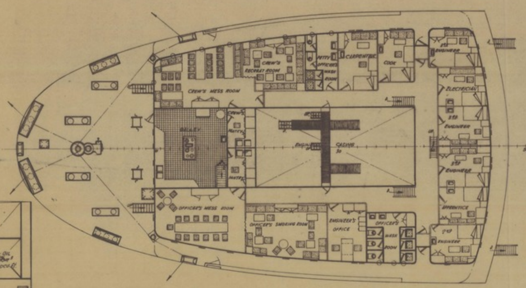
POOP DECK
