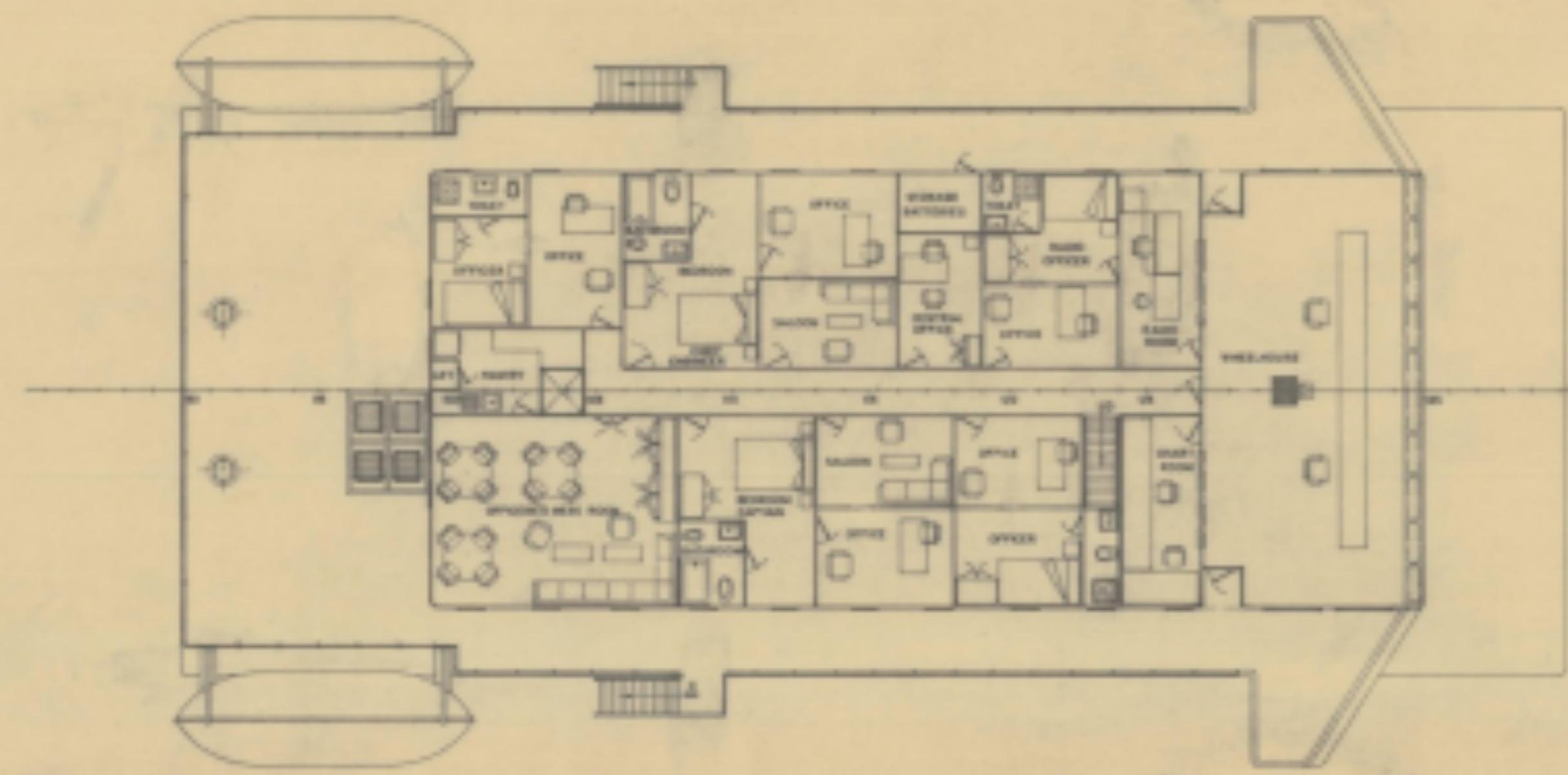
WHEELHOUSE DECK
