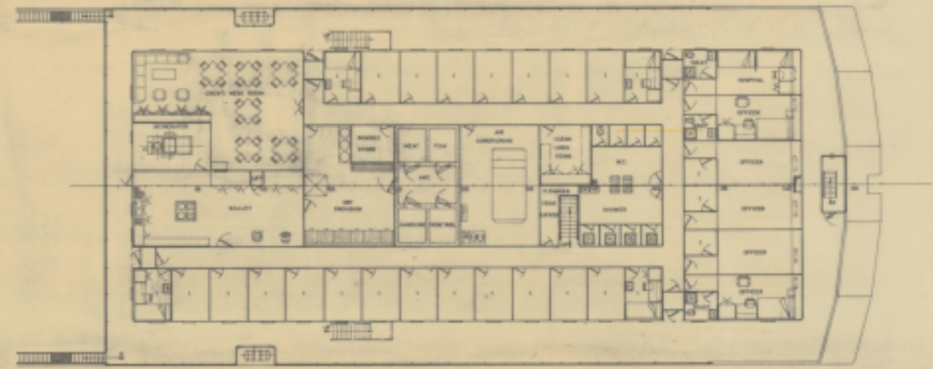
BOATS DECK
