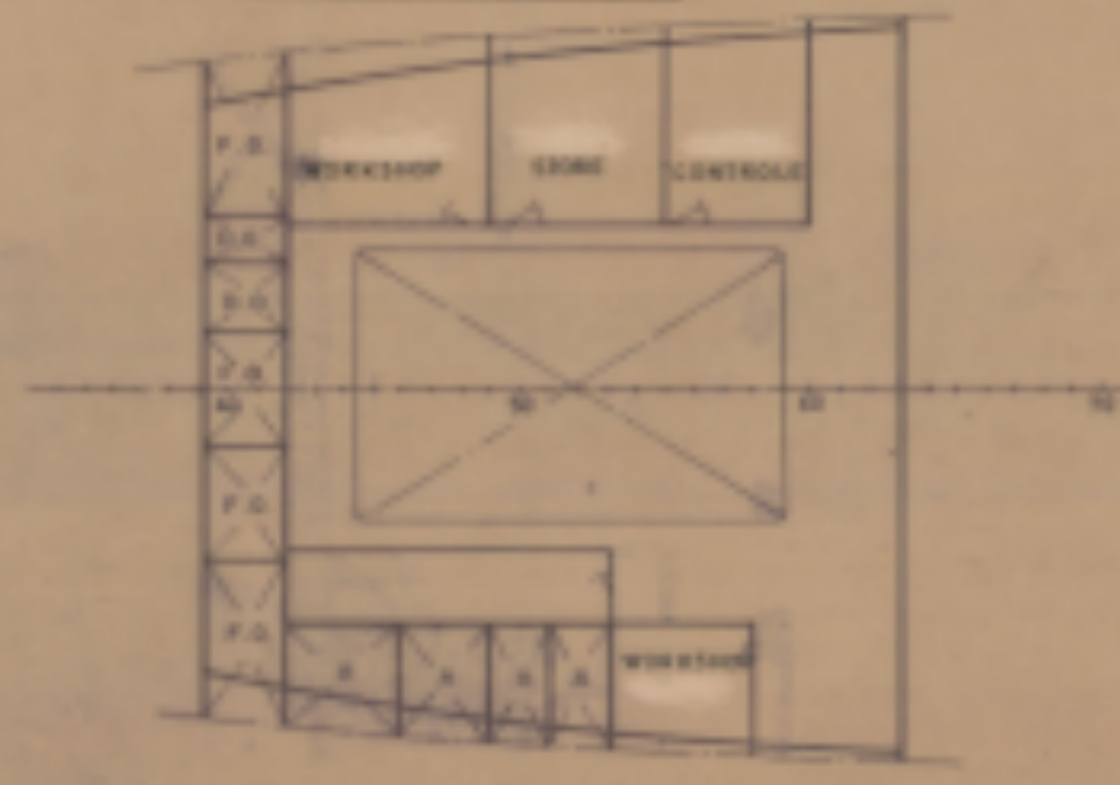
PLATAFORMA DEL MOTOR PLATFORM DECK ENGINE
