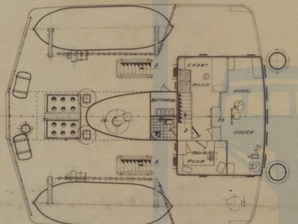
BRIDGE DECK
