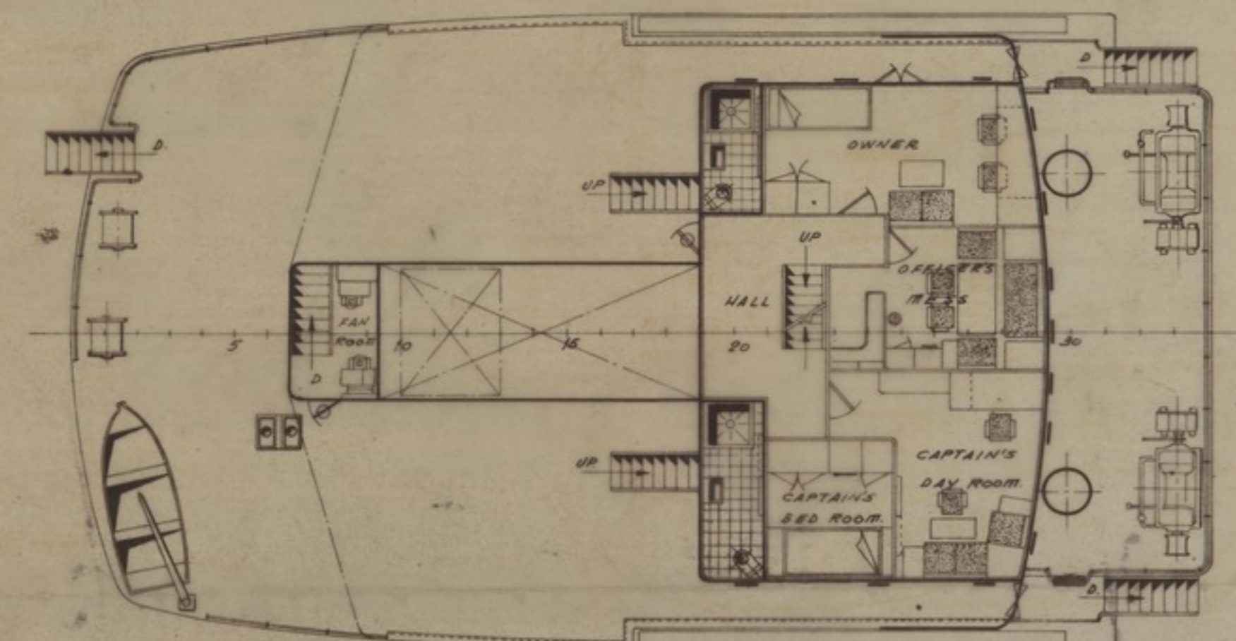
RAISED QUARTER DECK
