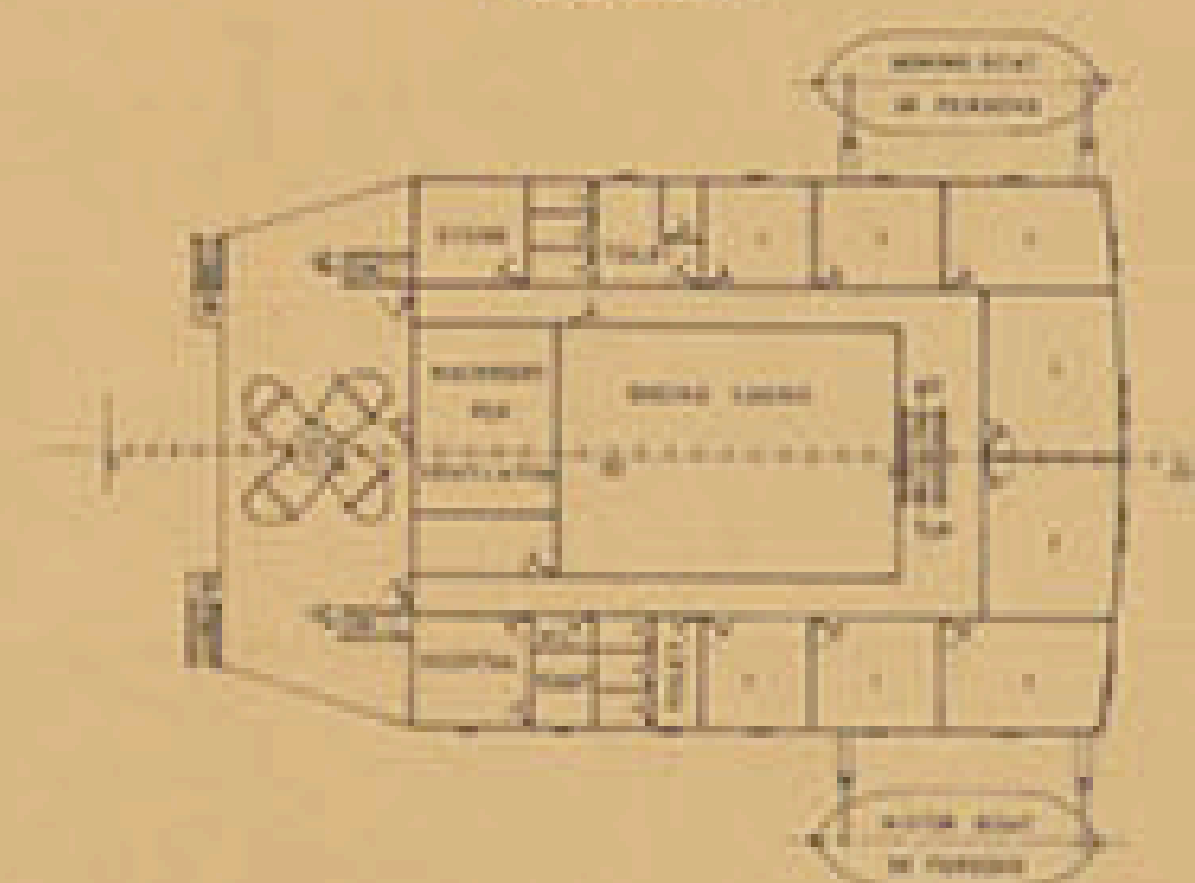
CUB. BOTES BOAT DECK
