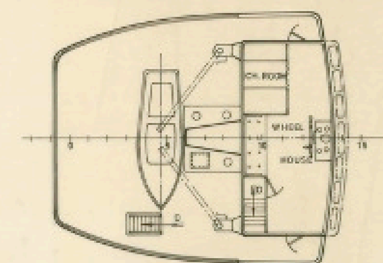
NAVIGATION BRIDGE DECK
