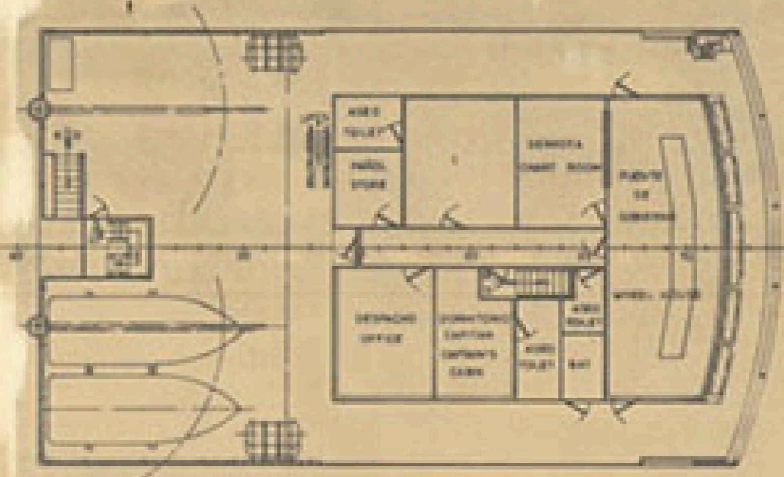
CUB. BOTES BOAT DECK
