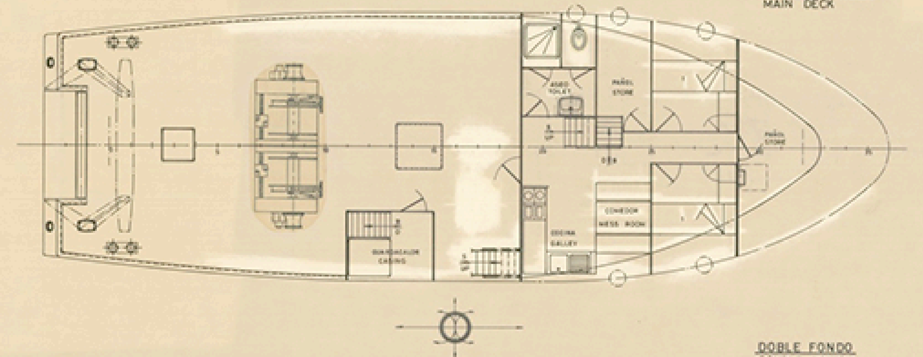
CUB. PRINCIPAL MAIN DECK
