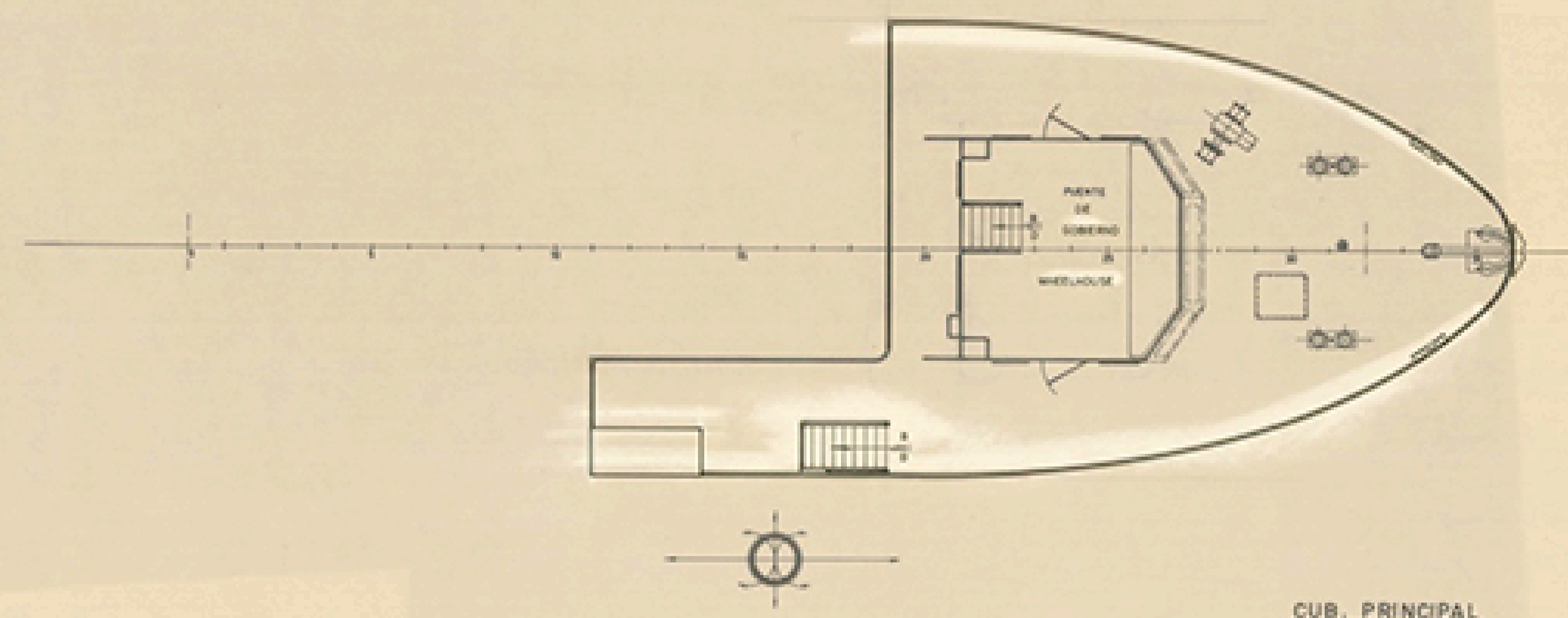
CUB. PRINCIPAL MAIN DECK
