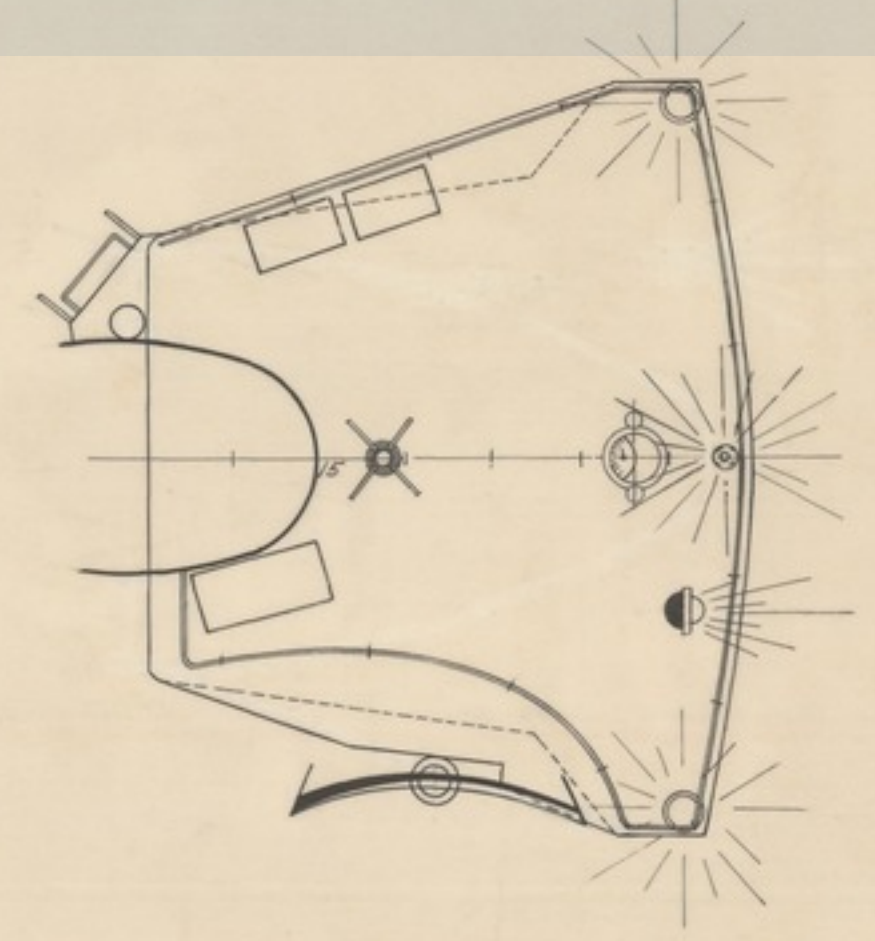
WHEEL HOUSE TOP
