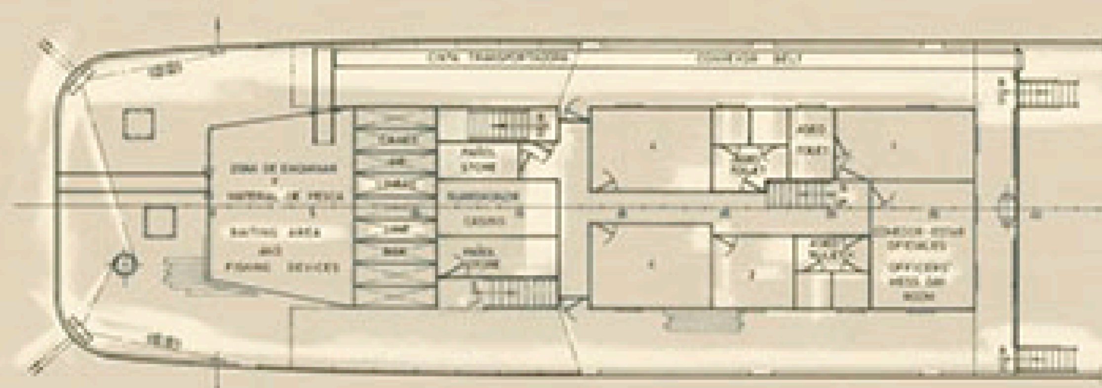
CUB. TOLOILLA POOP DECK
