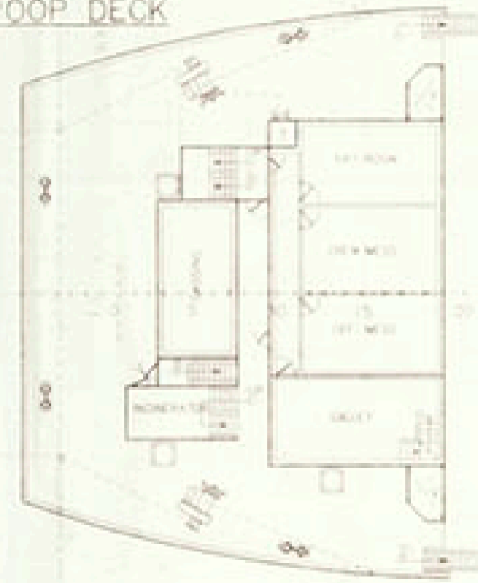
POOP DECK
