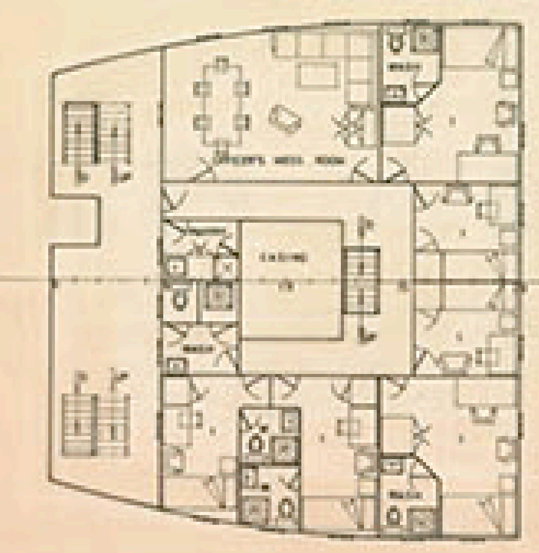
SUPERSTRUCTURE DECK
