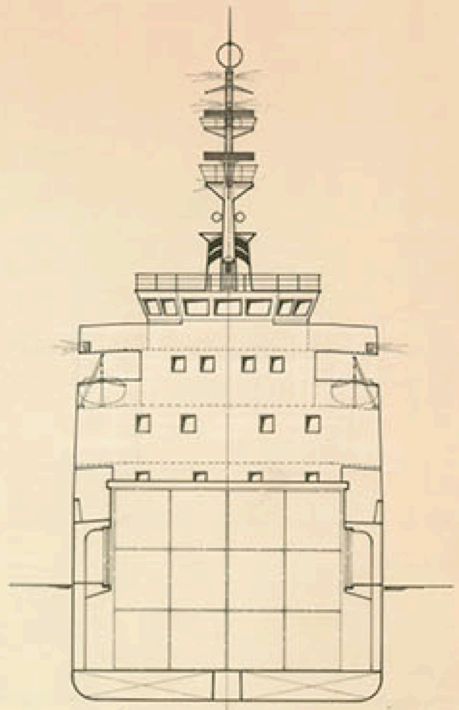
TRANSVERSE SECTION
