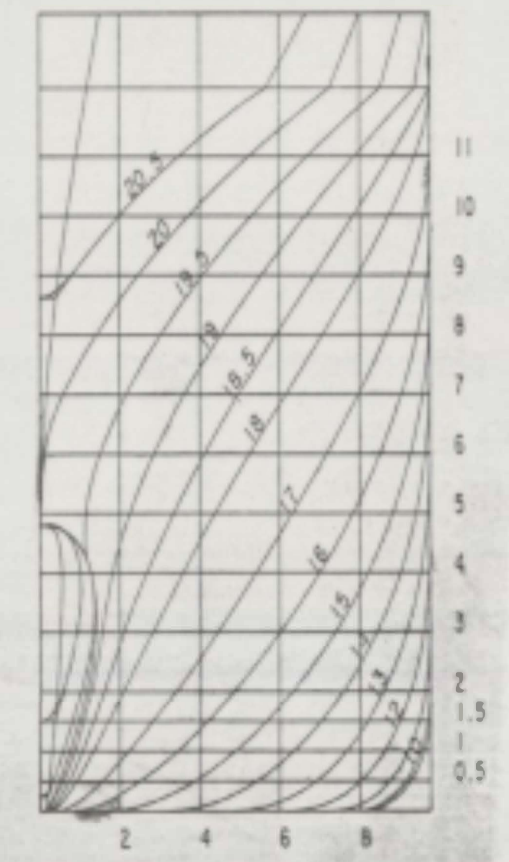
LINESPLAN FOR 250 PASSENGER FERRY
